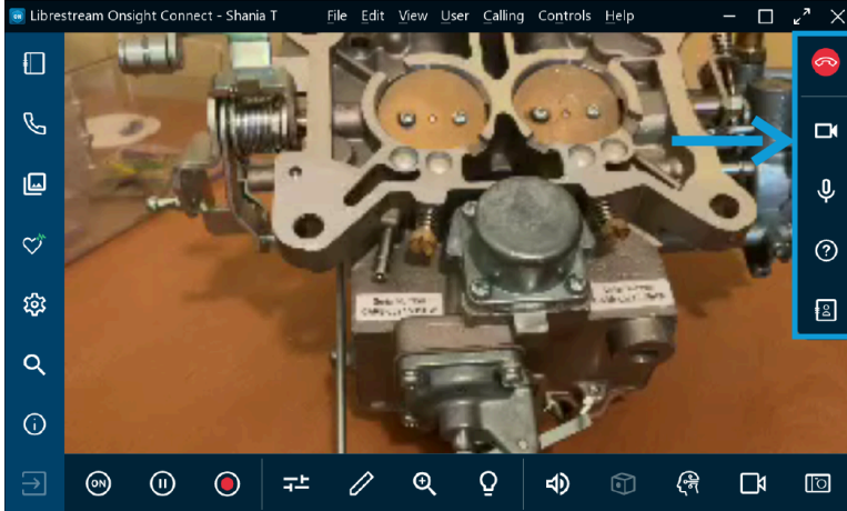
Figure 2-10 Right Toolbar
