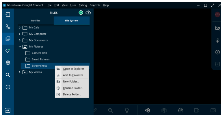
Figure 2-5 File Options
